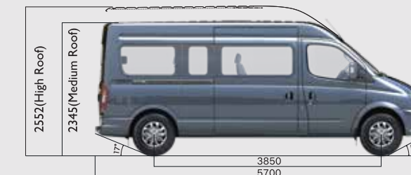
LWB Medium/High Roof
